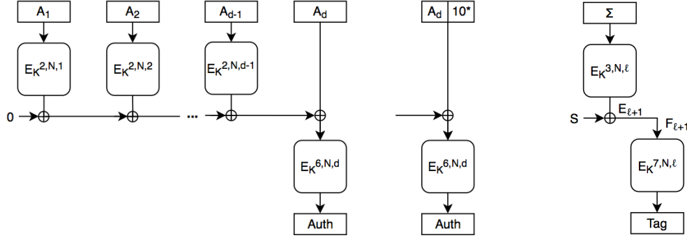
Figure 6.4.: (left) Associated Data Processing. (right) Tag Generation for Deoxys = , Joltik = and KIASU = .
