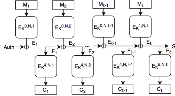
Figure 6.3.: Message Processing for Deoxys = , Joltik = and KIASU = .
