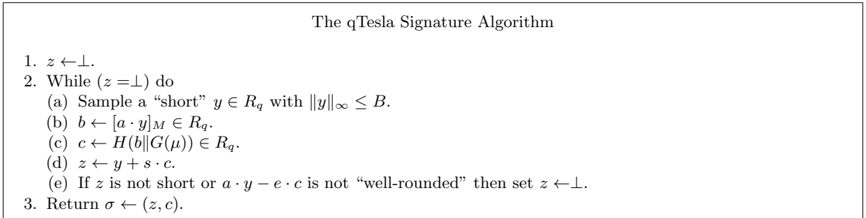
Figure 3. The qTesla Signature Algorithm
